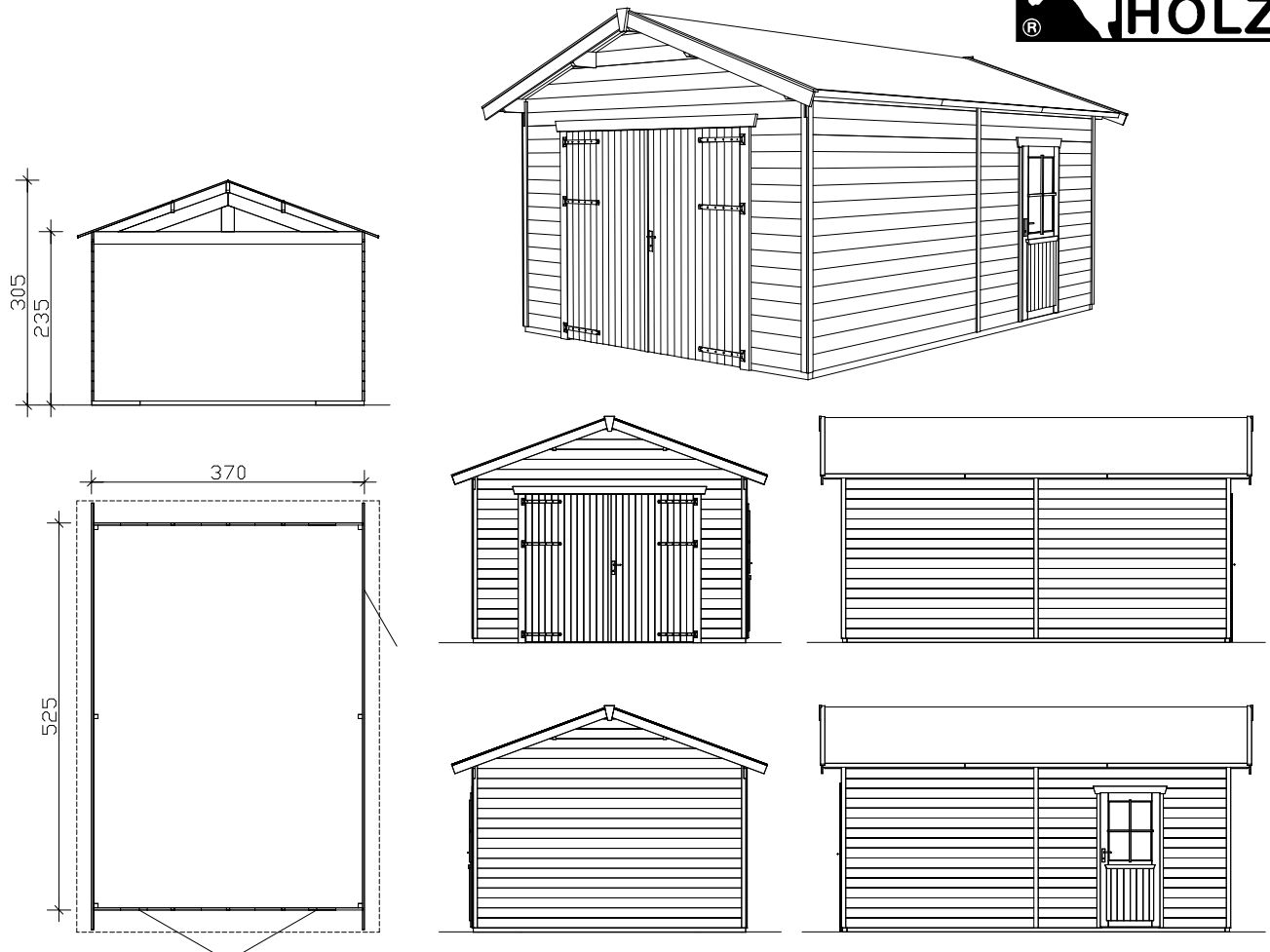
Floor plan, cross-section and elevations M 1:100
