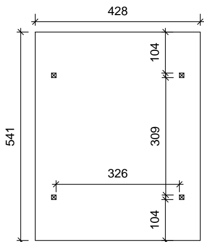
Ground plan
