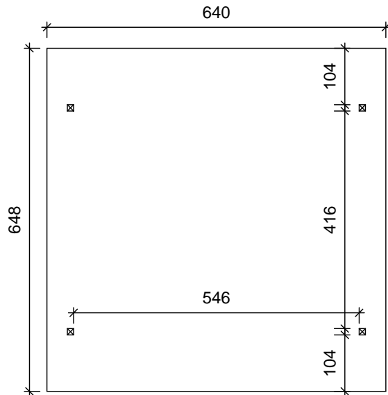
Ground plan
