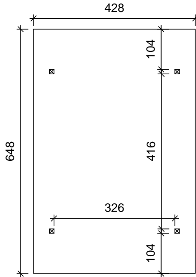
Ground plan
