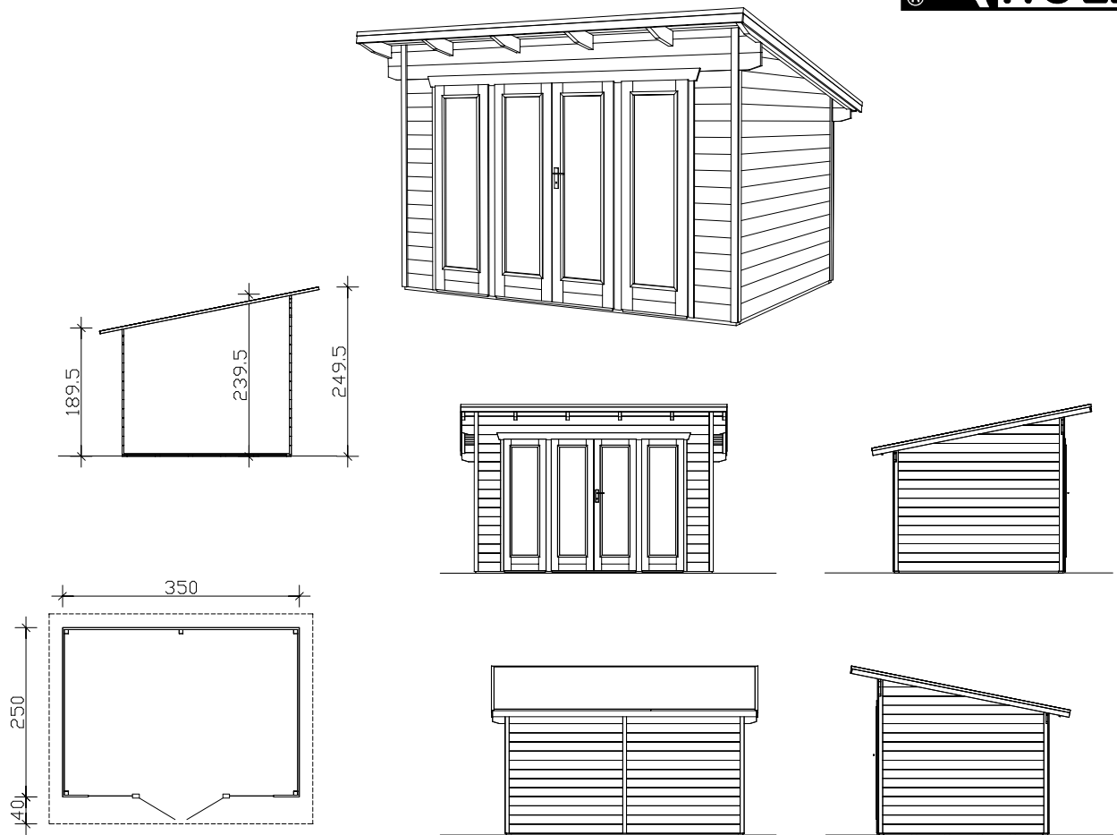
Floor plan, cross-section and elevations M 1:100
