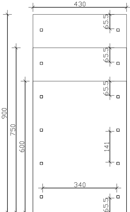
Ground plan
