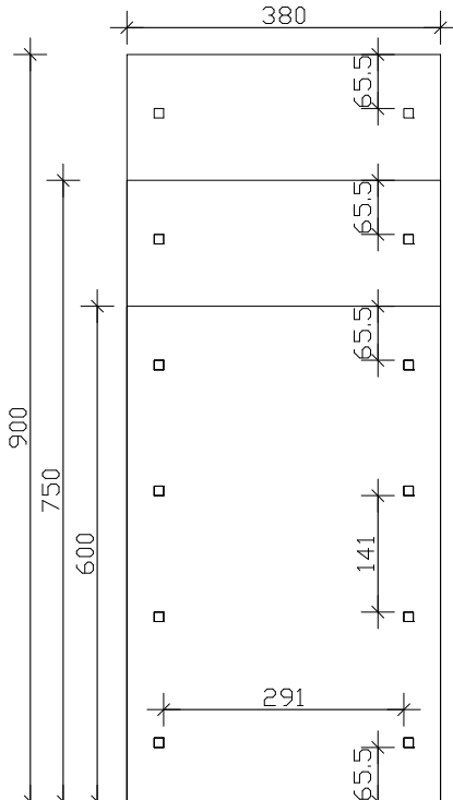
Ground plan
