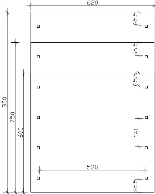
Ground plan
