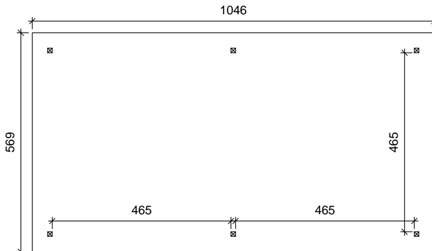
Groundplan
