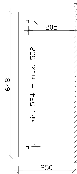
Floor plan
