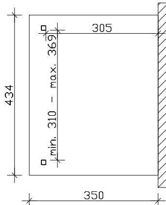
Floor plan
