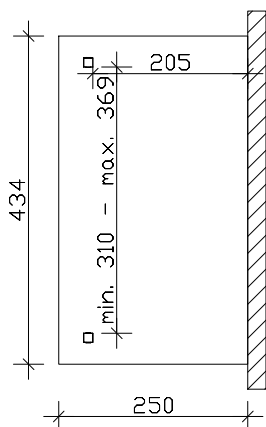
Floor plan
