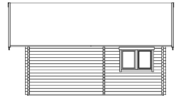
Floor plan, cross-section and elevations M 1:100
